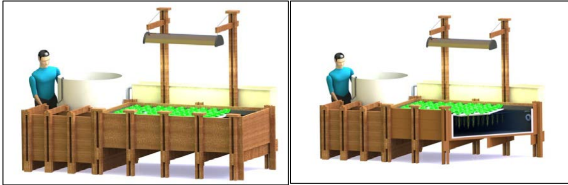
Figure 3. A 3-D drawing of the small aquaponics system (left). A cut-away view of the water tank for plants (right).
