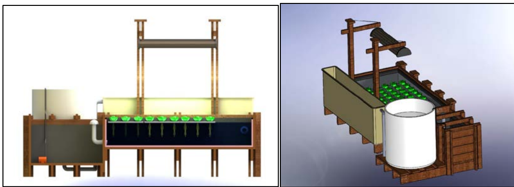
Figure 4. A cross-sectional view of the sump pump and plant tanks (left). A 3-D view from the rear showing the fish tank (cylinder) and the long rectangular tank for solids removal and bio-filter (right).
